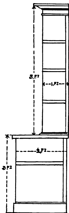
FIG. 38.—Wooden Wall Case with Ledged Base (Section 178).
